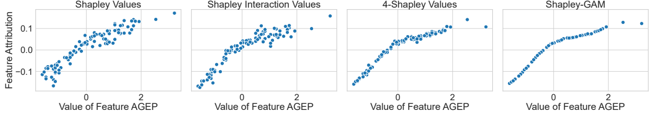
Figure 2: As n \rightarrow d , the n -Shapley Values provide increasingly precise representations of the component functions f_S of the Shapley-GAM. This figure depicts partial dependence plots of \Phi_{\text{AGEP}}^1 (Shapley Values, n = 1 ), \Phi_{\text{AGEP}}^2 (Shapley Interaction Values, n = 2 ), \Phi_{\text{AGEP}}^4 (4-Shapley Values, n = 4 ) and \Phi_{\text{AGEP}}^{10} (Shapley-GAM, n = d ). The leftmost partial dependence plot is the usual plot that is often used in order to visualize Shapley Values (Lundberg et al., 2020) (the plot depicts the original Shapley Values for the observations in the test set). It takes the often observed form where the Shapley Values are scattered around an overall functional relationship. Theorem 4 and Theorem 6 make this intuition precise by specifying how the Shapley Values are related to the component functions of the Shapley-GAM. The middle and right plots illustrate that as we move towards higher-order explanations, interaction effects can be appropriately represented. As a consequence, the partial dependence plots of individual feature attributions approach the component functions of the Shapley-GAM. In this example, the function f is a KNN classifier on the Folktables Income classification task. Appendix Figure K.8 depicts the partial dependence plots of all other features.
